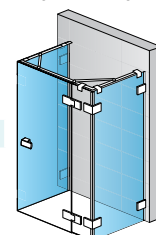
ME13AD + MET1AG + MET3AD + 2x RAM.E10
